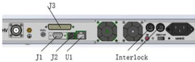
1U/2U chassis communication interface
